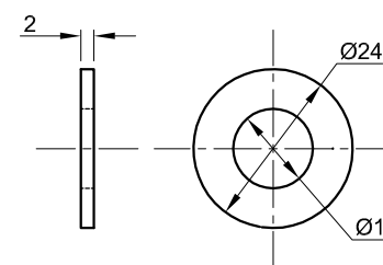
WASHER [6]
