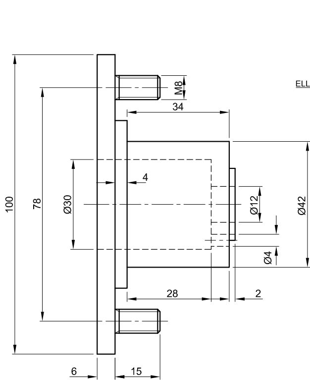
SEAL [2]
