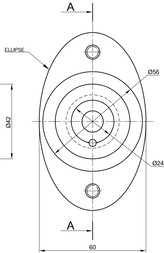
BASE [3]
